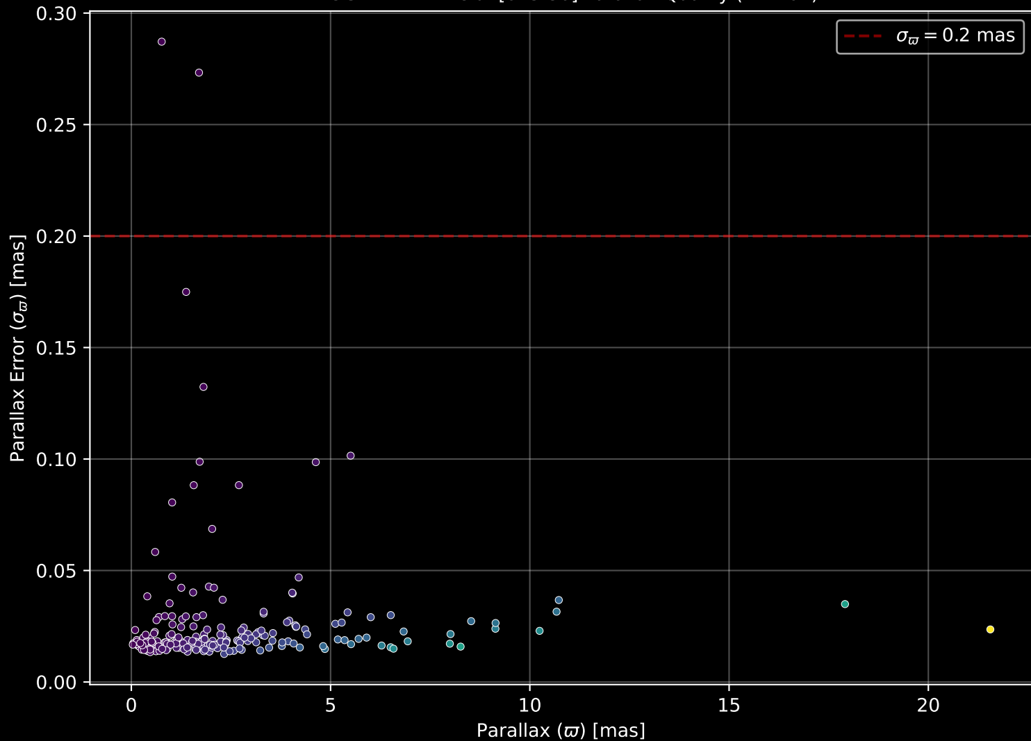
APOGEE DR17 Field: [075-30] Parallax Quality (n= 207)
