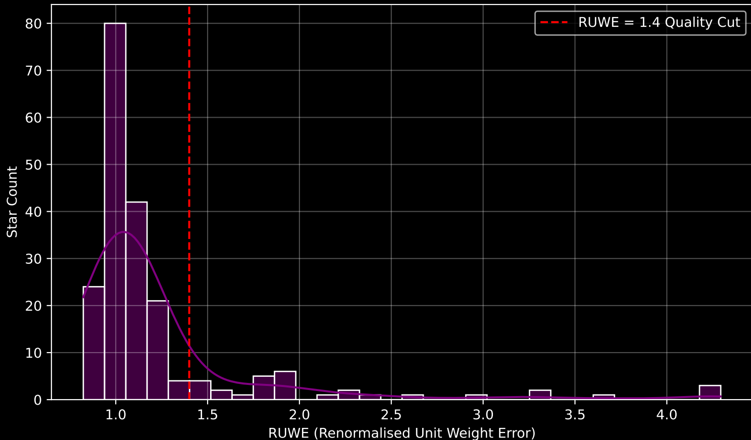
GAPOGEE DR17 Field [075-30] RUWE Distribution (n= 201)
