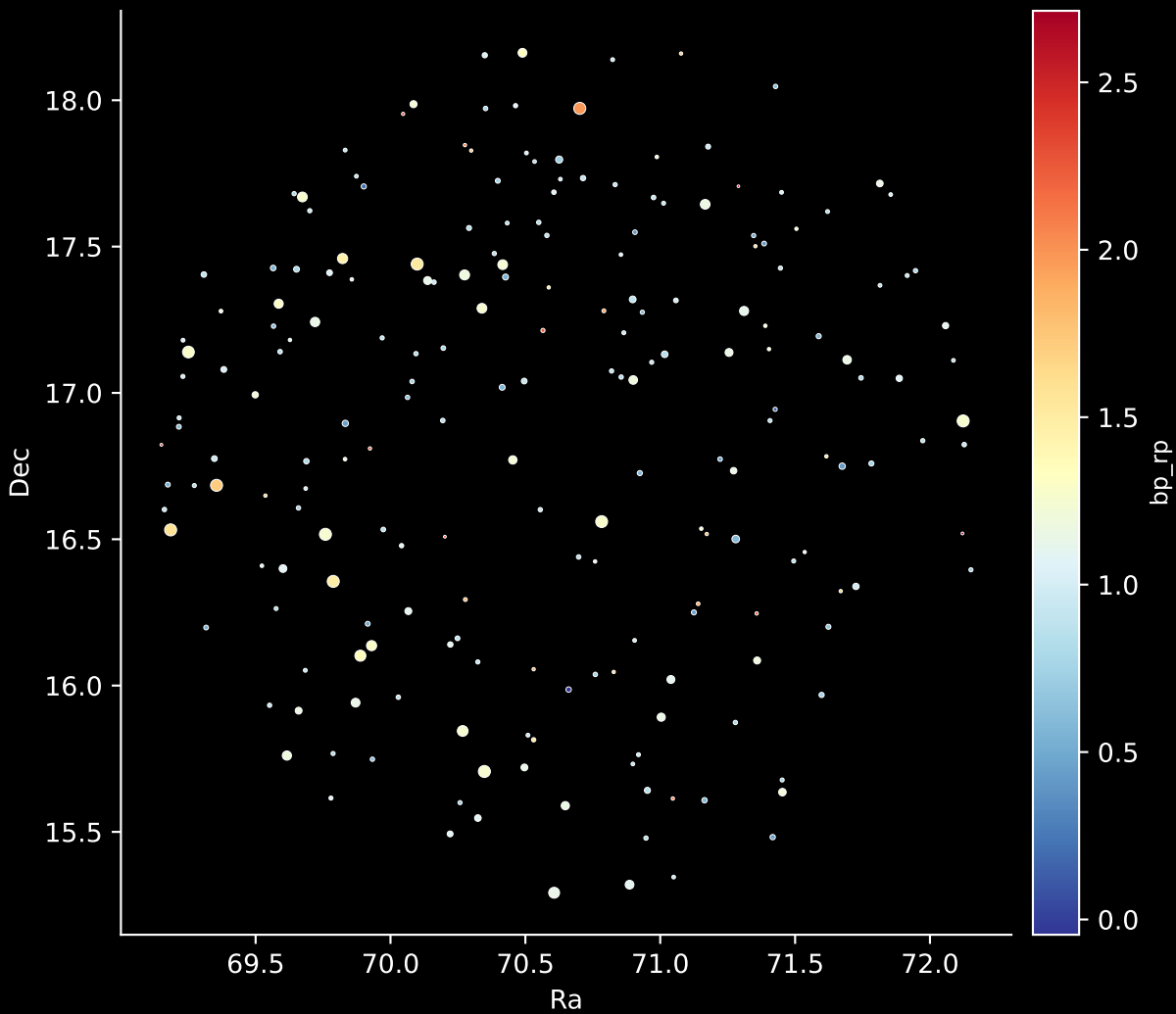
APOGEE DR17 Field: [075-30] Stars: 207
