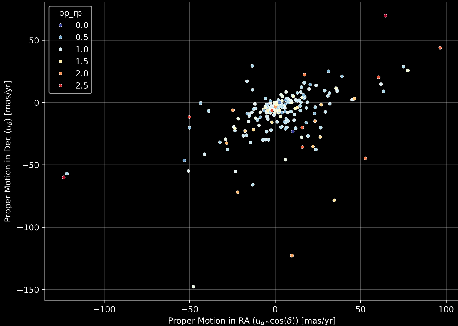
APOGEE DR17 Field: [075-30] Proper Motion Diagram (n= 207)
