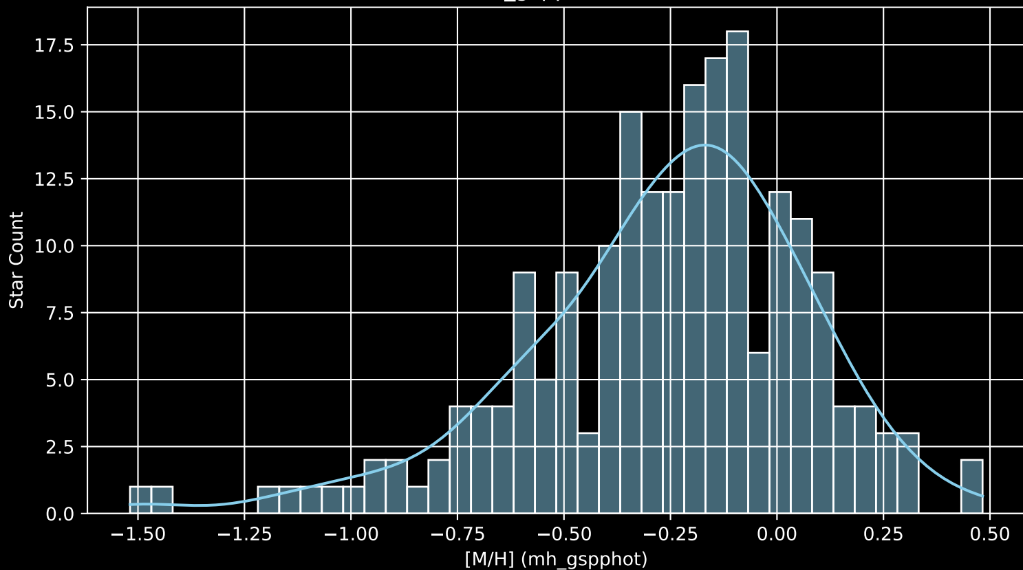
APOGEE DR17 Field: [075-30 [M/H] (mh_gspphot) (n= 206)
