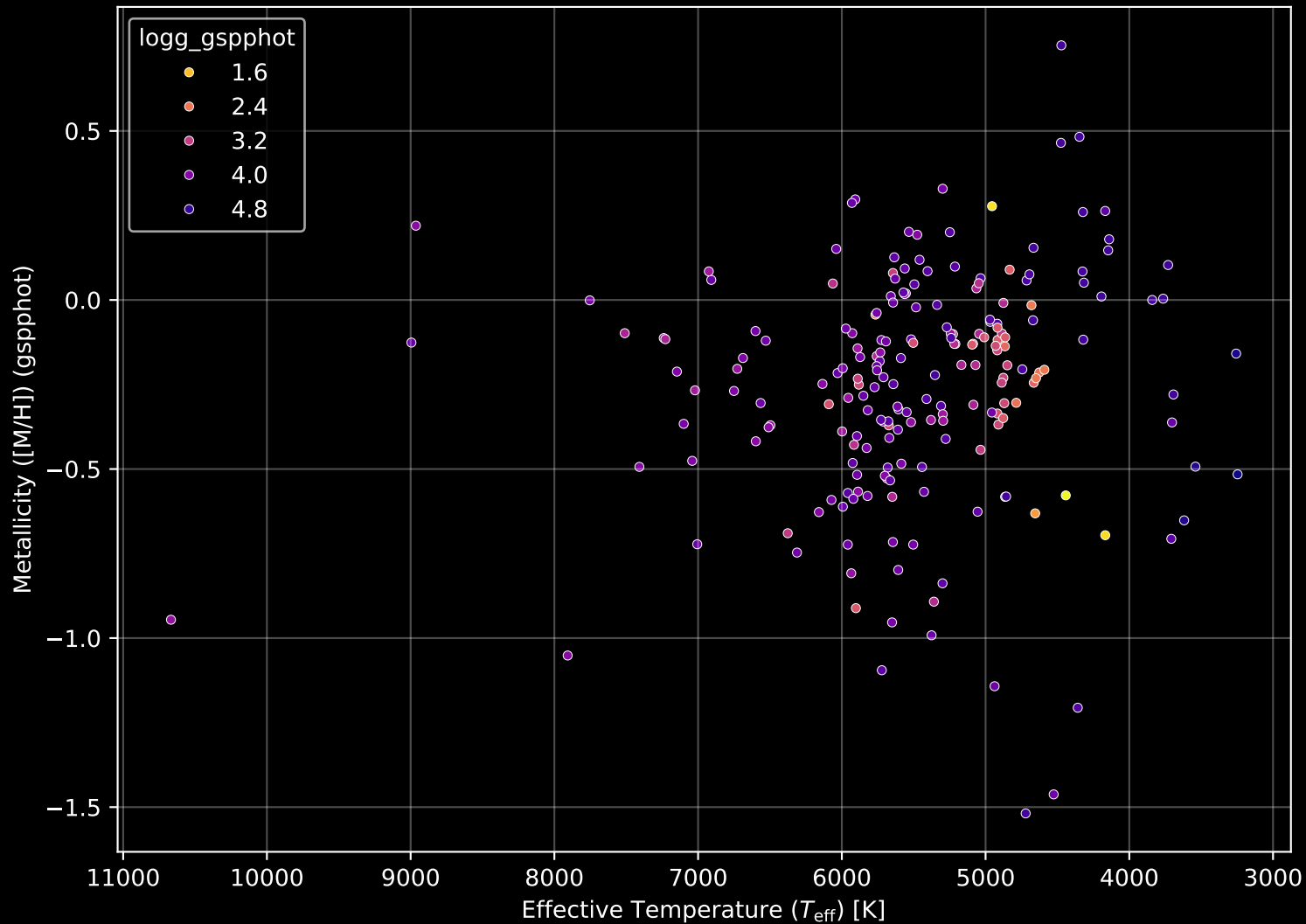
APOGEE DR17 Field: [075-30] Stellar Population Parameters (n= 207)
